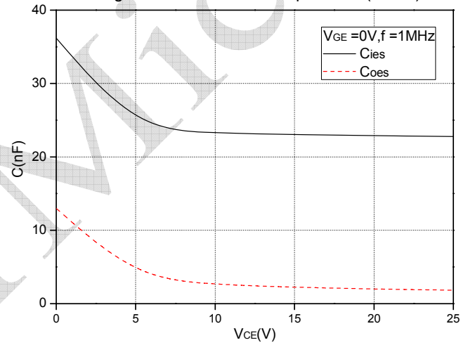
Fig.10 Capacitance Characteristics
