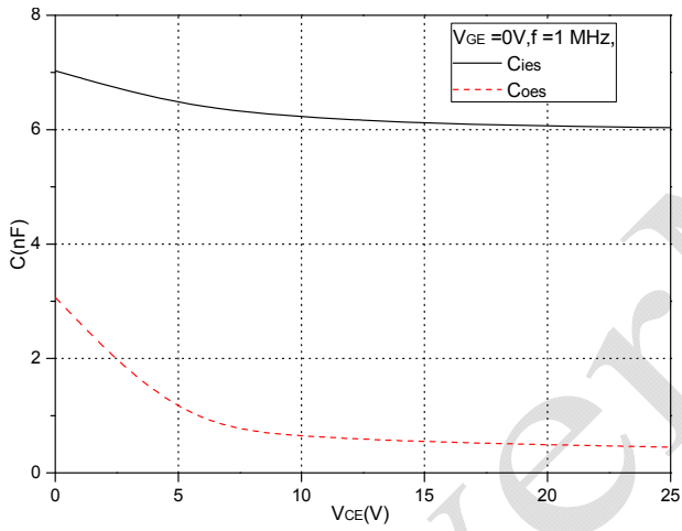
Fig.9 Capacitance Characteristics
