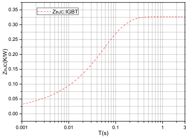
Fig.7 Transient Thermal Impedance (IGBT)
