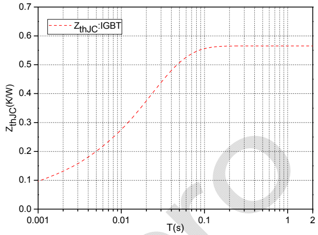
Fig.8 Transient Thermal Impedance IGBT (Inverter)
