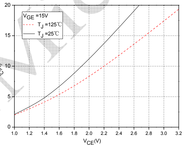
Fig.10 Typical Saturation Voltage Characteristics (Brake-Chopper)
