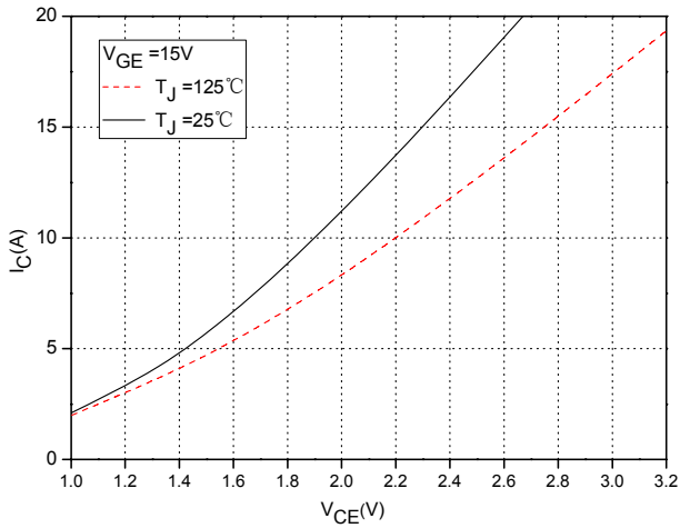
Fig.1 Typical Saturation Voltage Characteristics (Inverter)
