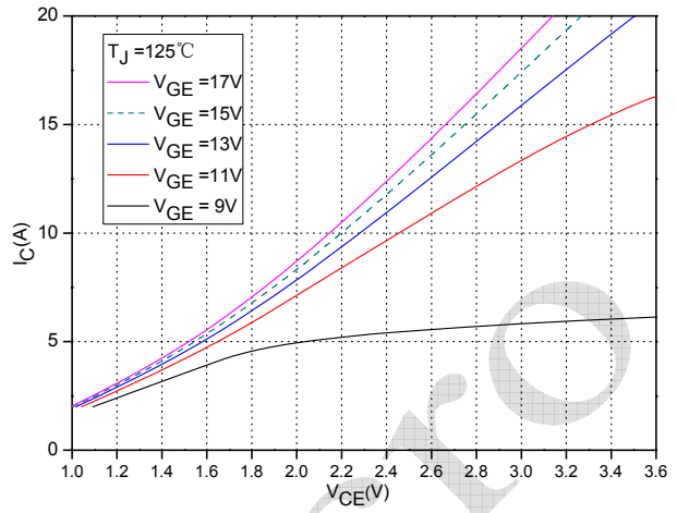
Fig.2 Typical Output Characteristics (Inverter)
