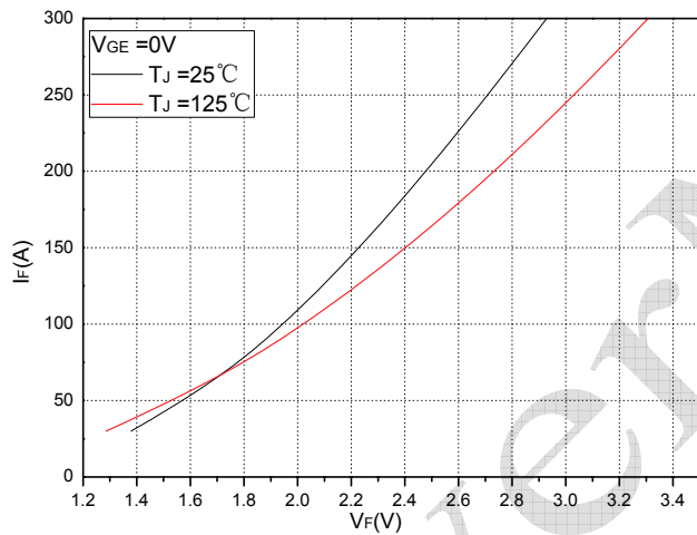
Fig.3 Forward Characteristics of FWD (Reverse)
