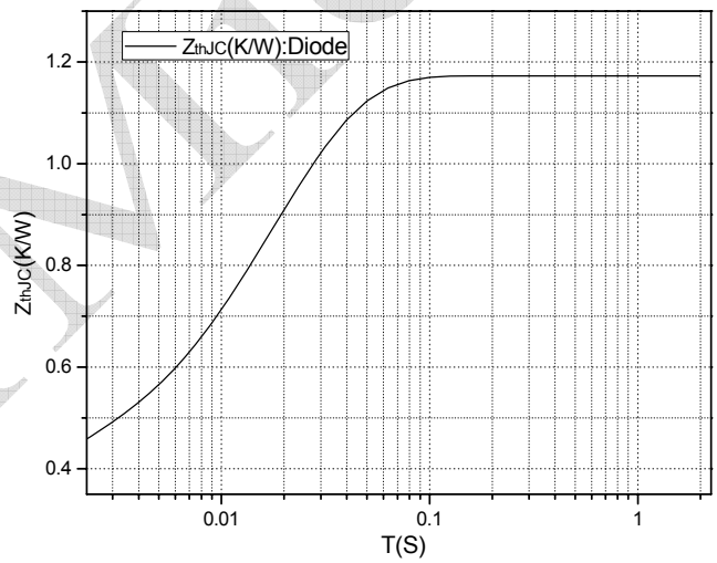
Fig.10 Transient Thermal Impedance Diode
