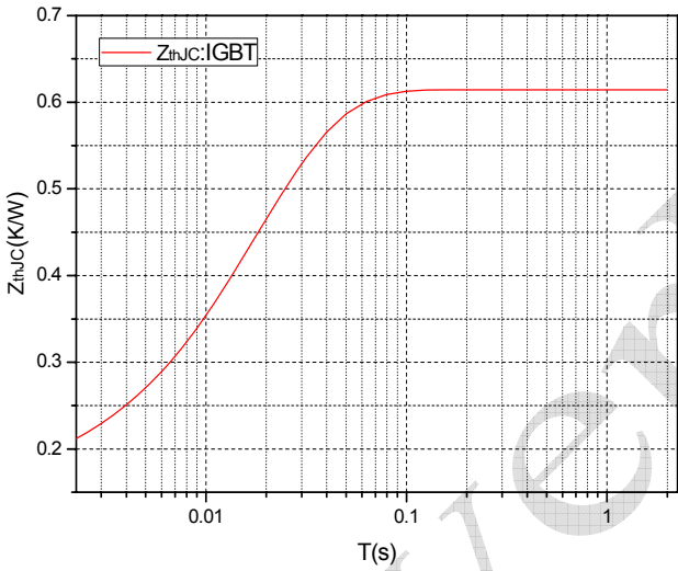
Fig.9 Transient Thermal Impedance IGBT
