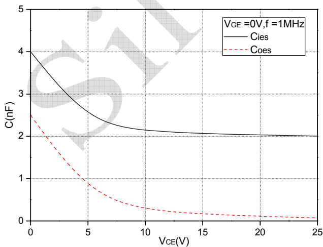
Fig.11 Capacitance Characteristics
