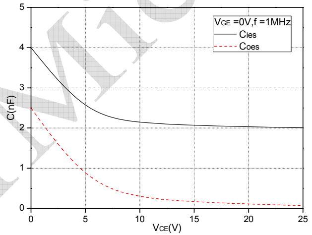
Fig.4 Capacitance Characteristics
