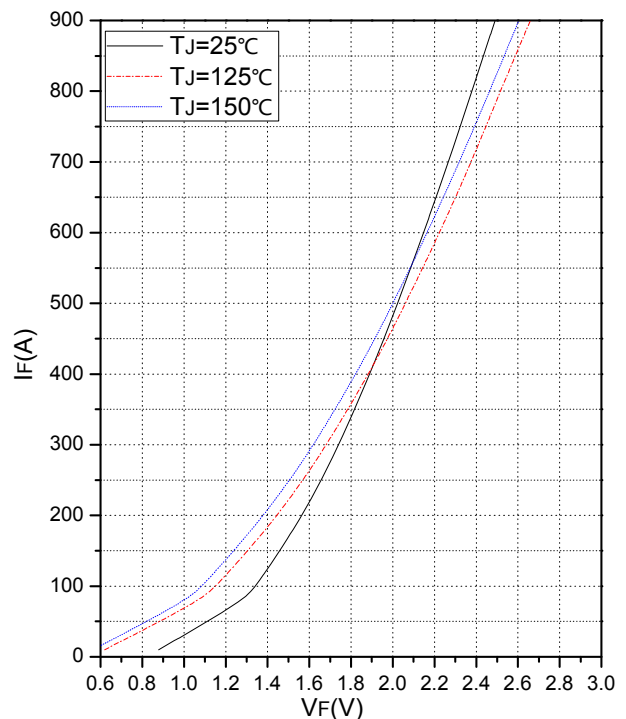
Fig.4 Forward Characteristics of Brake-Chopper Diode
