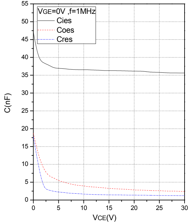
Fig.16 Capacitance Characteristics
