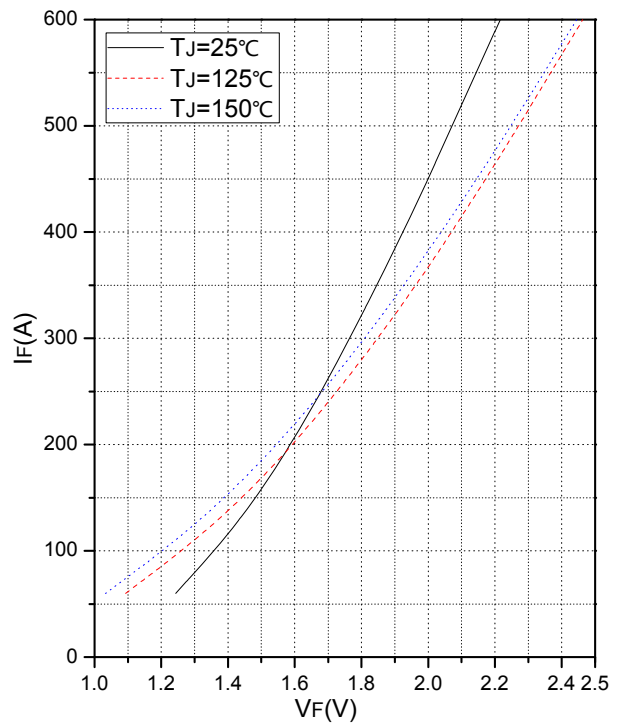
Fig.14 Forward Characteristics of Reverse Diode
