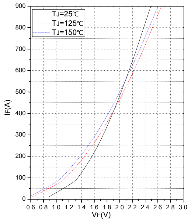
Fig.4 Forward Characteristics of Brake-chopper Diode
