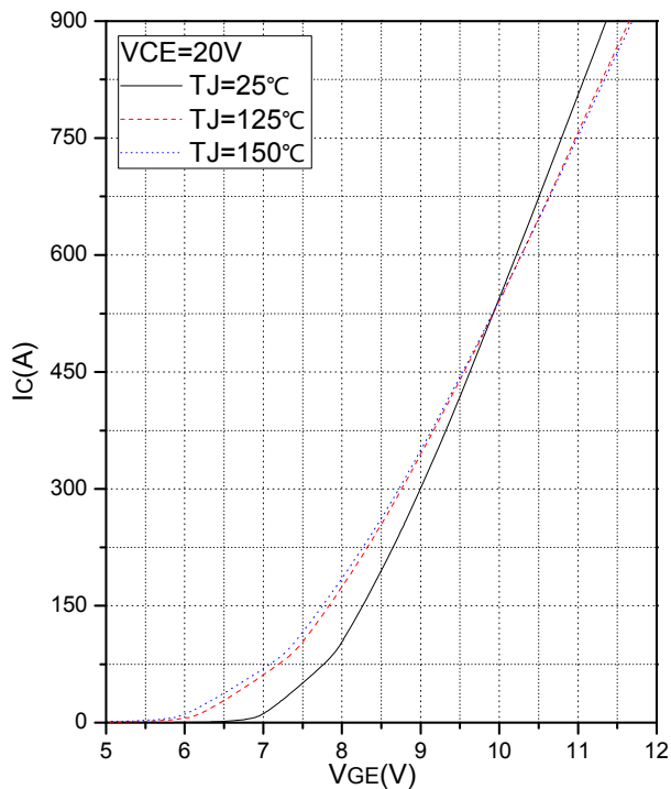
Fig.3 Transfer Characteristic
