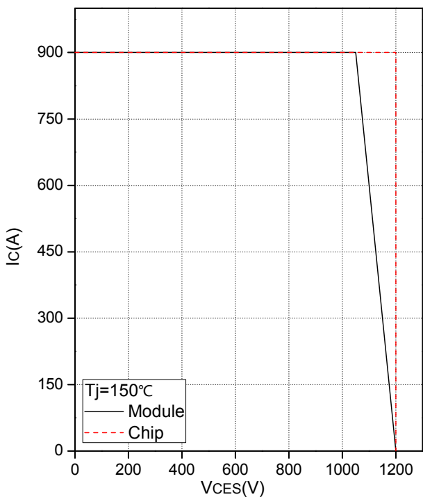
Fig.15 Reverse Bias Safe Operation Area (RBSOA)
