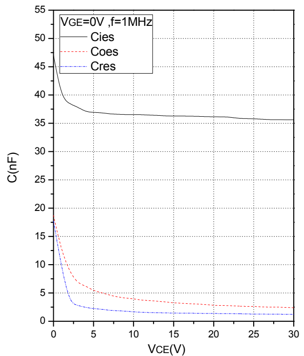
Fig.16 Capacitance Characteristics
