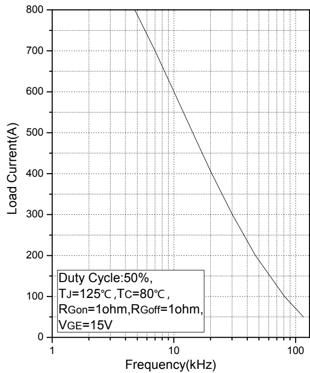
Fig.12 Typical Load Current vs. Frequency
