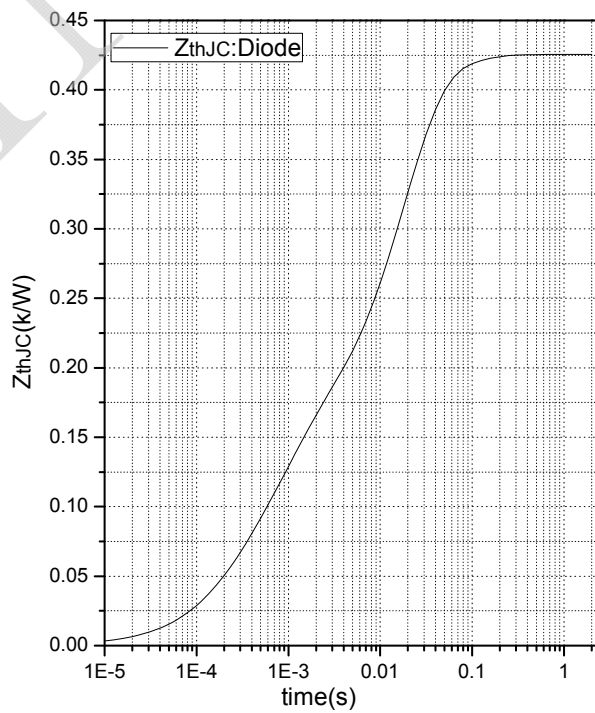
Fig.8 Transient Thermal Impedance (Diode-Chopper)
