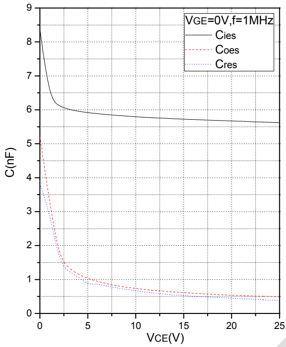
Fig.9 Capacitance Characteristics
