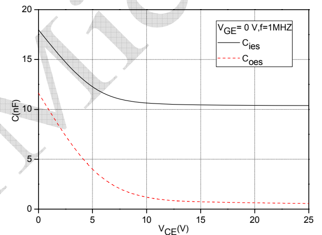
Fig.4 Capacitance Characteristics
