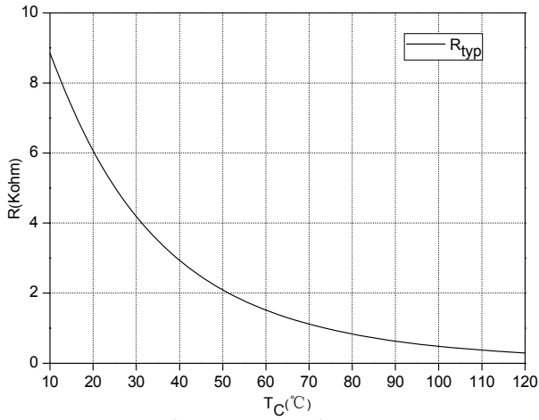
Fig.7 NTC Temperature Characteristics
