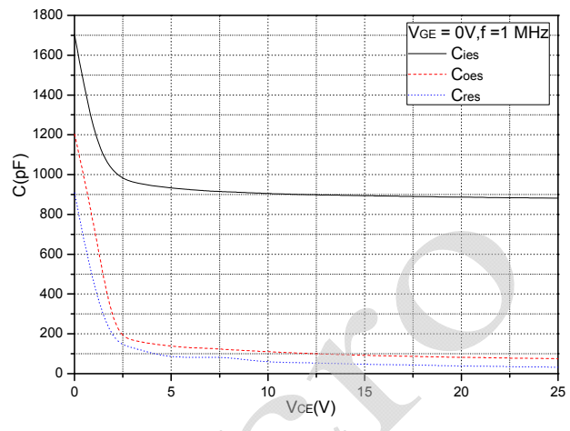
Fig.14 Capacitance Characteristics
