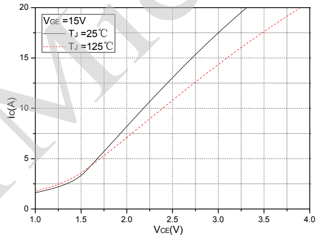
Fig.10 Typical Saturation Voltage Characteristics (Brake-Chopper)
