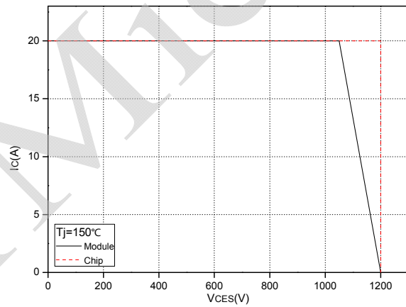
Fig.4 Reverse Bias Safe Operation Area (RBSOA)
